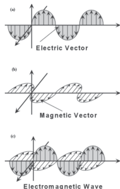
Figure 1. (a) and (b) the electric and the magnetic component of a electromagnetic wave, are shown respectively. (c) The electromagnetic wave is composed of an electric and a magnetic component. These components are perpendicular to each other and to the direction of propagation of the wave.
